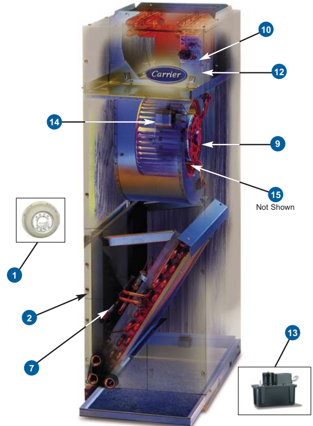
Typical Air Handling Unit
